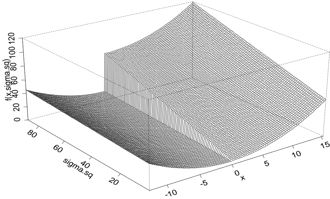
Figure 1: Simulation experiment. The volatility surface f(x, \sigma^2) = 5 + 0.2x^2 + (0.75\mathbf{1}_{\{x>0\}} + 0.11\mathbf{1}_{\{x\leq 0\}})\sigma^2 ; note the asymmetry depending on the sign of x .
