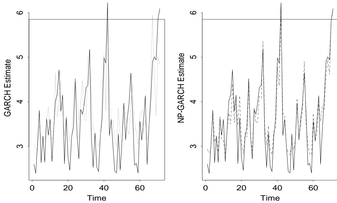
Figure 4: Simulation experiment. For an arbitrary section of 70 observations from the simulated time series, the left-hand plot shows true volatility (solid line) compared with a parametric GARCH(1,1) estimate (dotted line) and the right-hand plot shows true volatility compared with the nonparametric GARCH estimate obtained after a final smooth (dashed line).
